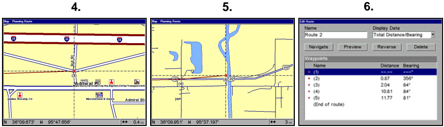
Route creation sequence, continued: Fig. 4. Point (3) set at on-ramp turn. Fig. 5. Waypoint (4) set at highway exit to frontage road leading to river. Waypoint (5) ends the route at a tree stand in the hunting area. Fig. 6. Press EXIT to save the route and you return to this screen.
