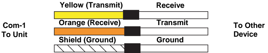
Com-1 wiring to exchange information with another device.
